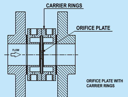
ORIFICE PLATE WITH CARRIER RINGS
