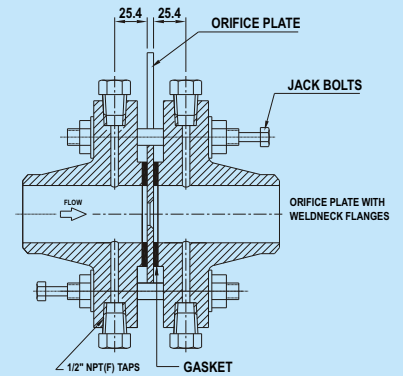
ORIFICE PLATE WITH WELDNECK FLANGES
