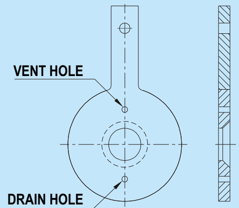
SQUARE EDGED CONCENTRIC ORIFICE PLATE
