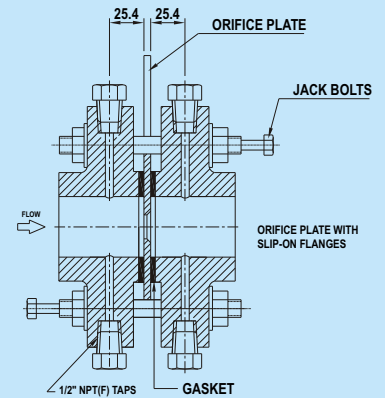
ORIFICE PLATE WITH SLIP-ON FLANGES
